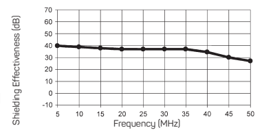
EMP shielding (MEOB.96_049 ELM)
