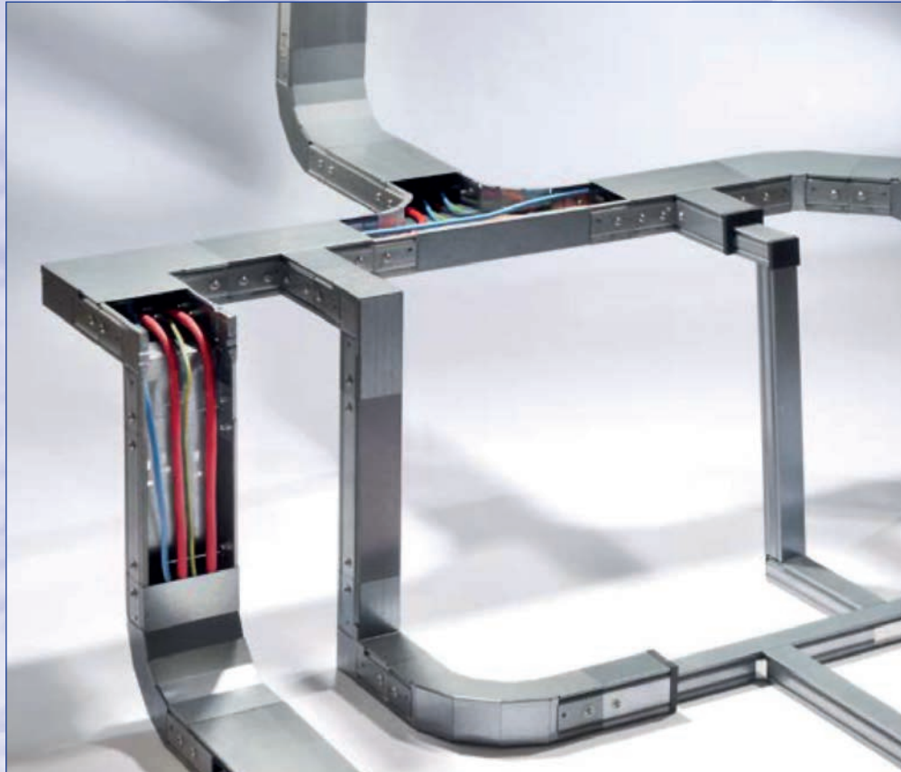
Pflitsch Industriekanal in Edelstahl Pflitsch Industrial Trunking in stainless steel Chemin de câble Pflitsch Industriel en acier inoxydable
